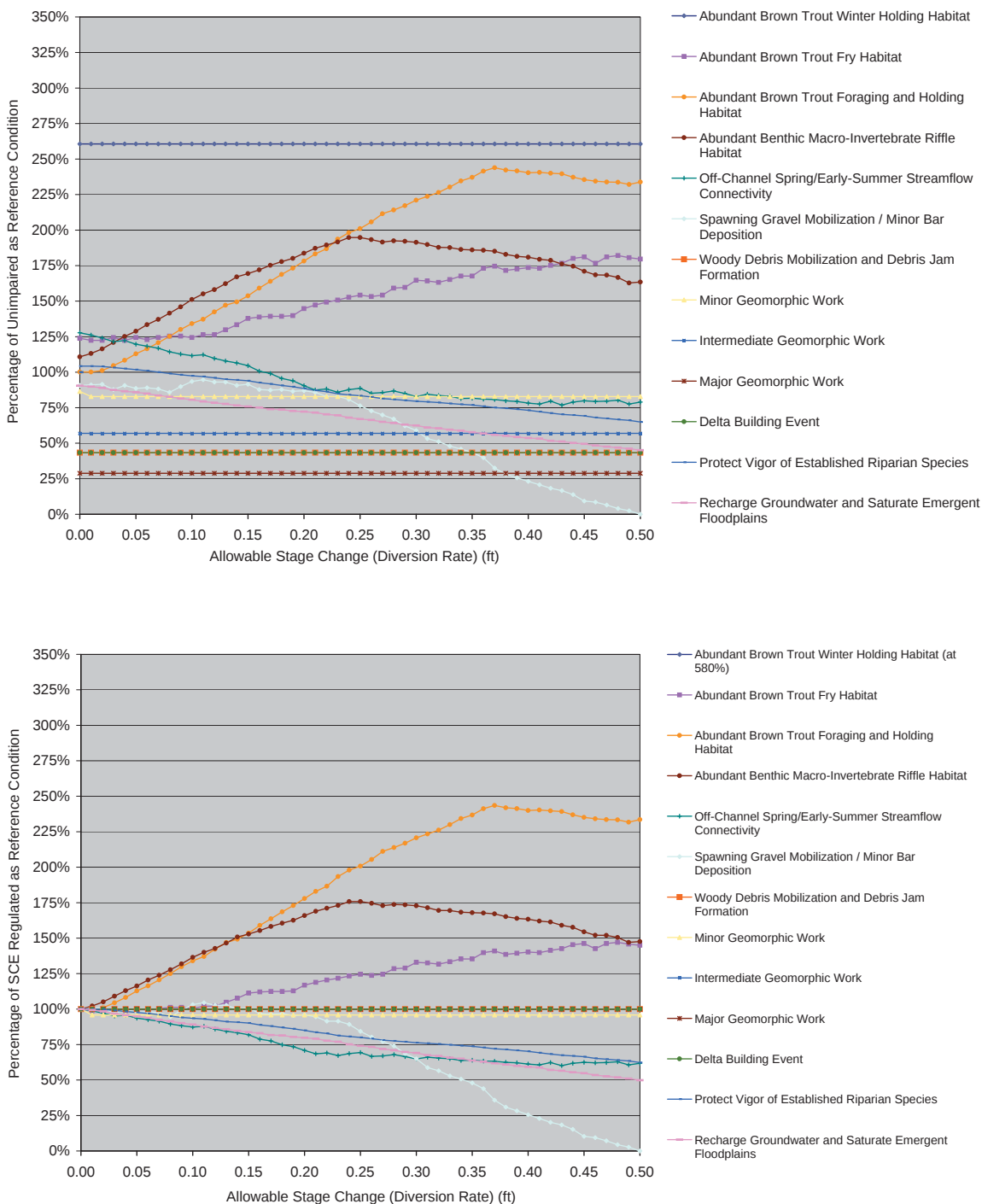
Figure 4-5. NGD analysis for Lee Vining Creek using the percent of unimpaired Lee Vining Creek flows as reference condition (above) and the percentage of SCE regulated Lee Vining Creek above Intake flows as reference condition (below). For each ‘desired ecological outcome’ the number of days thresholds were exceeded is computed, and then divided by the reference condition number of days. This computation was performed for each incrementally larger diversion rate, to produce a reference condition curve for each desired ecological outcome.
