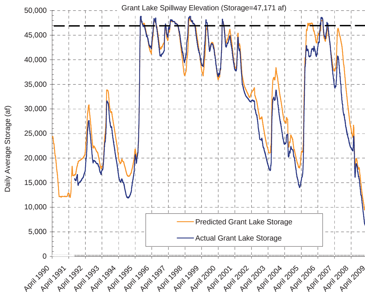
Figure 3-3. Actual vs Predicted Grant Lake Reservoir storage volume for RYs 1990 to 2008 used for hydrologic simulations. Once the model was calibrated to best predict GLR storage, the “predicted historic” storage volume was used as the basis for comparison in simulated diversion and export scenarios.
