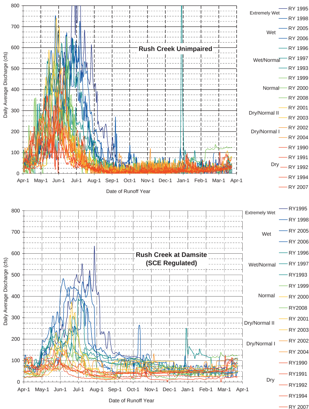
Figure 5-1. Annual hydrographs for Rush Creek Runoff (computed unimpaired) and Rush Creek at Damsite (SCE regulated) for RYs 1990 to 2008 showing patterns in annual hydrograph components and the range of variability in different runoff year types.
