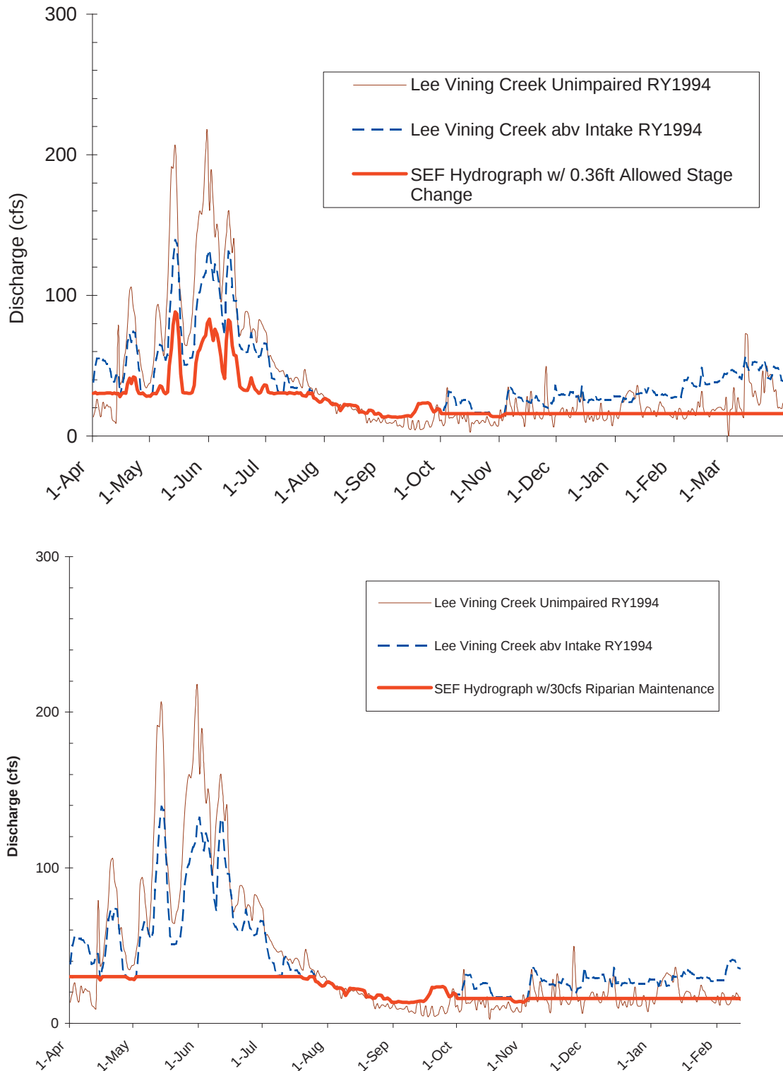
Figure 9-5a-b. Lee Vining Creek annual hydrograph for RY1994 as an example of alternative diversion strategies applied in Dry and Dry-Normal runoff years during the spring snowmelt diversion season, using (a) higher diversion rates derived from an 'Allowable Stage Change' of 0.36 ft (instead of 0.2 ft stage change used for other runoff year types), and (b) allowing a spring bypass flow of 30 cfs from April 1 to September 30.
