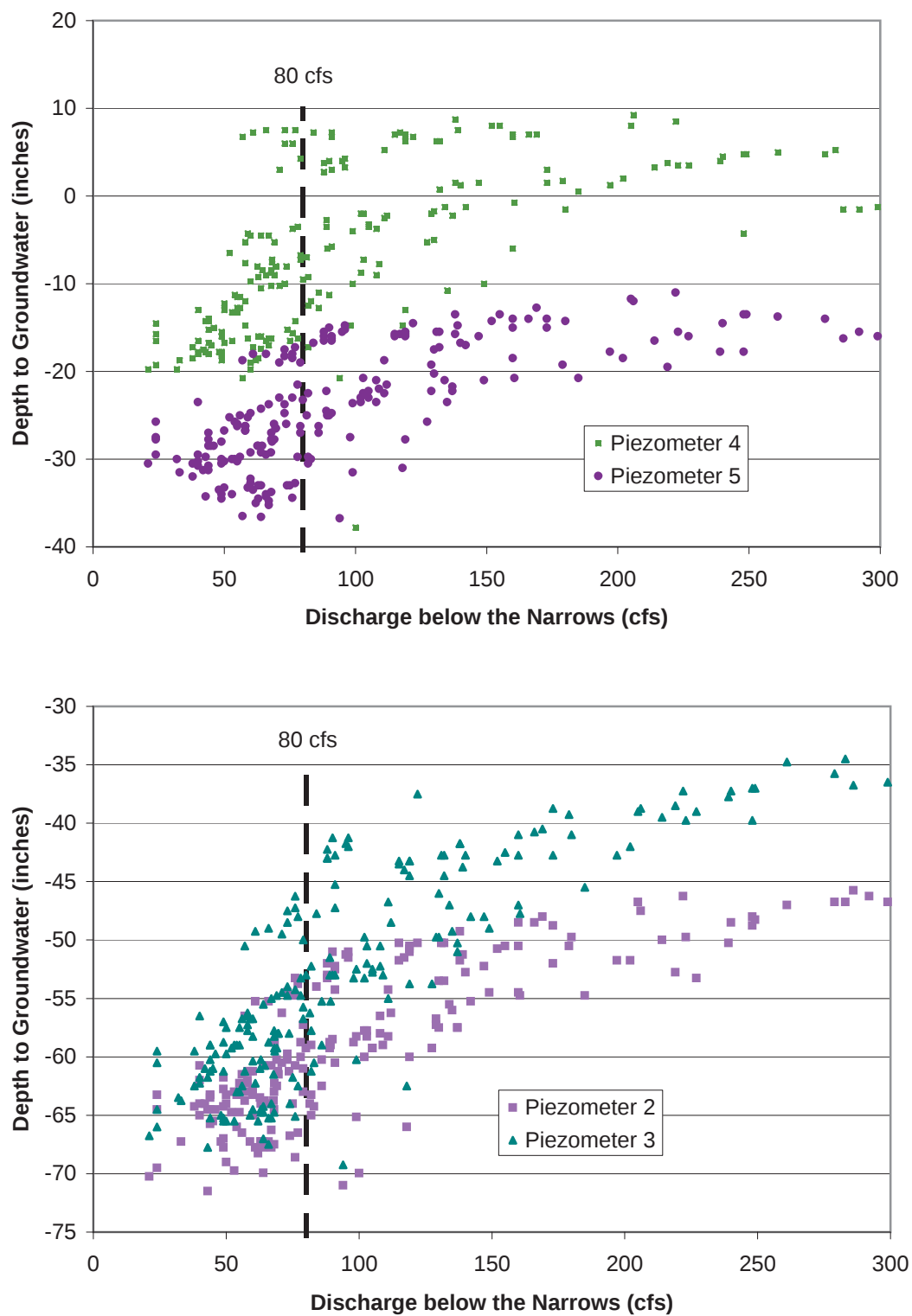
Figure 9-3. Groundwater elevations for the lower Rush Creek 10-Channel interfluvial piezometers measured from RY1995 to 2008 by the Mono Lake Committee. The data scatter show a trend in decreasing groundwater elevation with reduced discharge below the Narrows.
