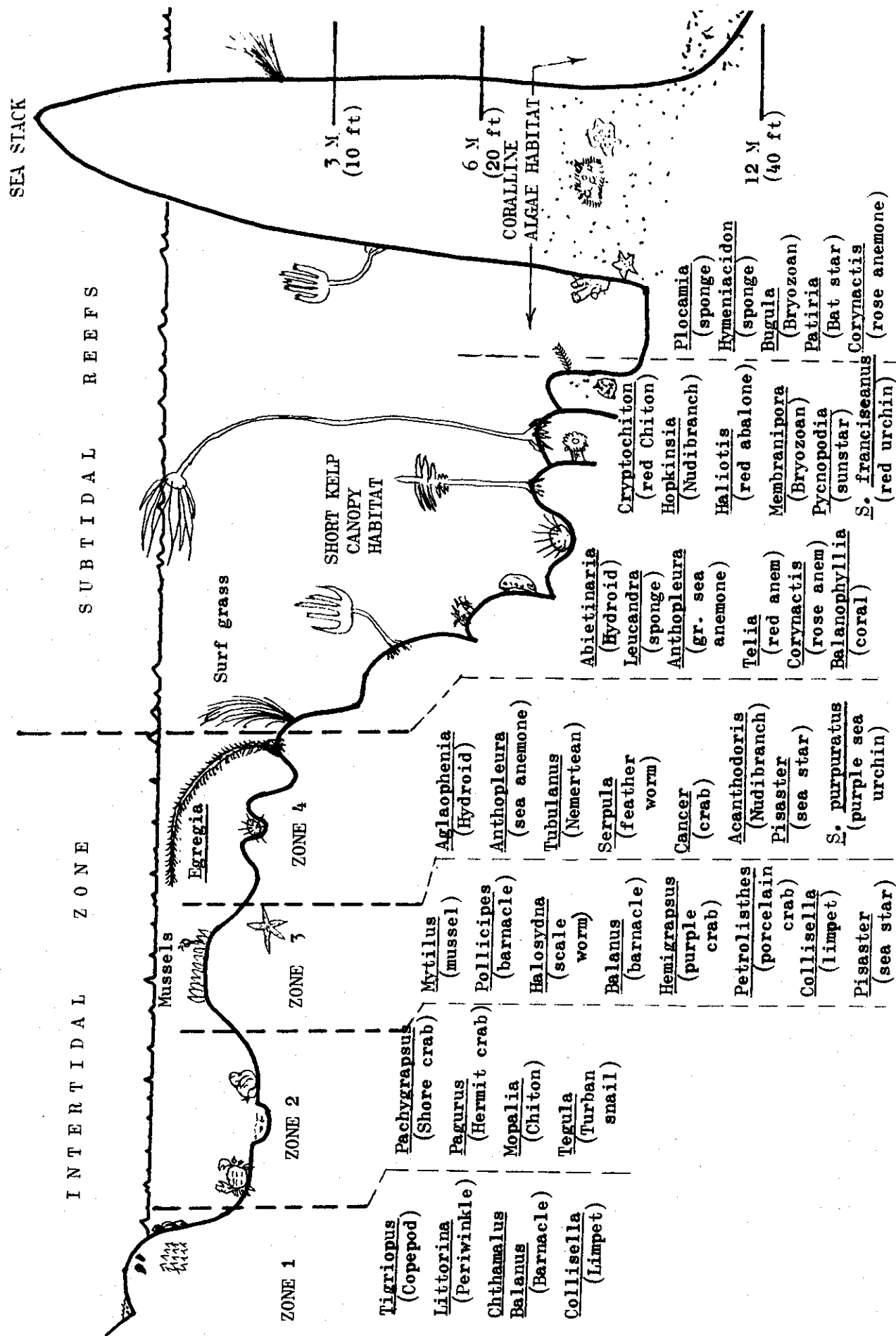
FIGURE 15. GENERAL DEPTH DISTRIBUTION OF INDEX INVERTEBRATES, DOUBLE POINT
